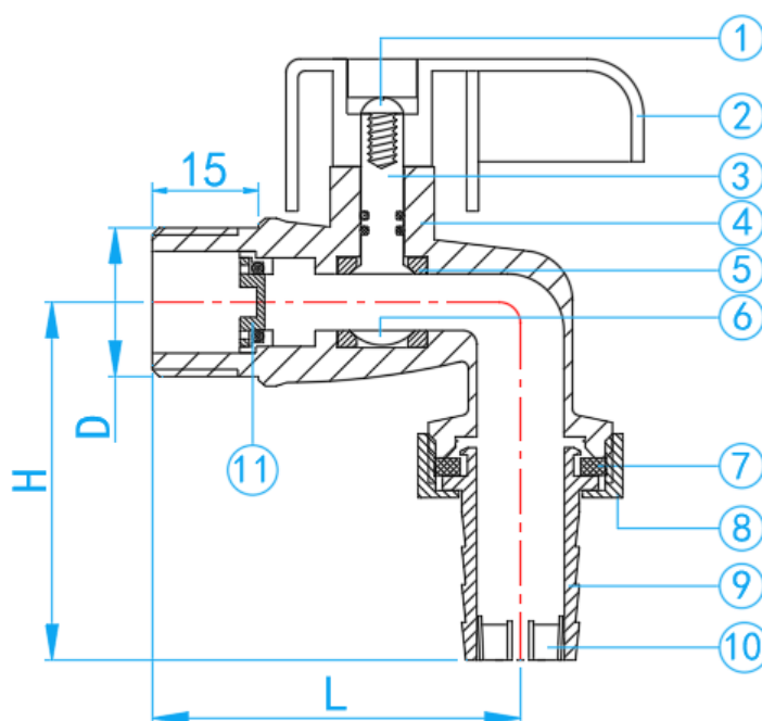
CROSS SECTION
